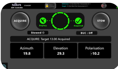
1:1 BUC control screen on RM150 ACU
